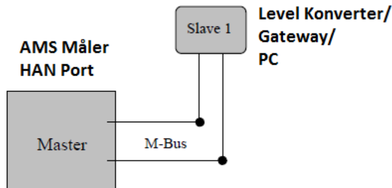
Fig. Block diagram showing principle of the M-Bus System
